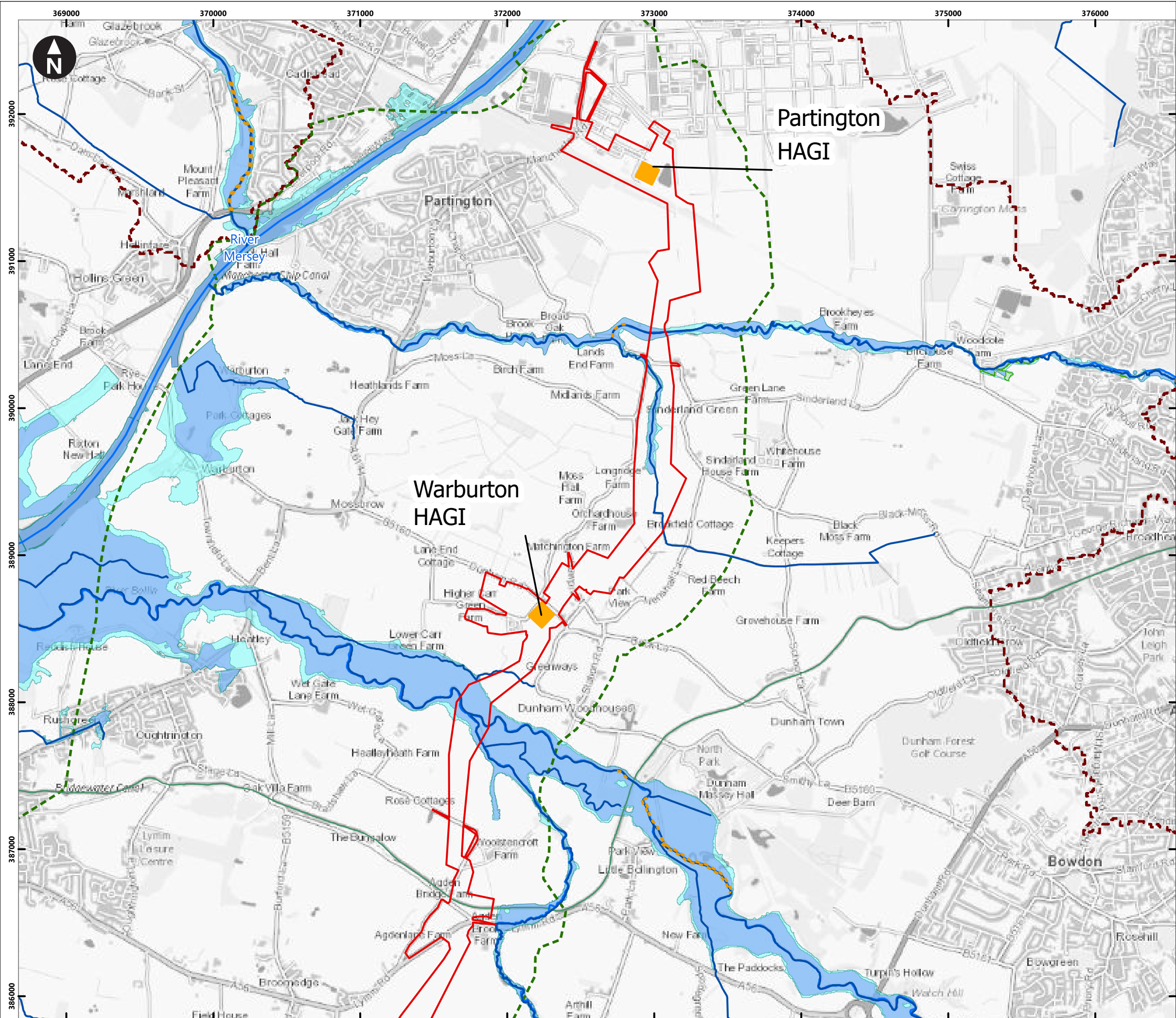
Figure 7.7 Environment Agency Flood mapping for Planning Sheet: 1 of 10
