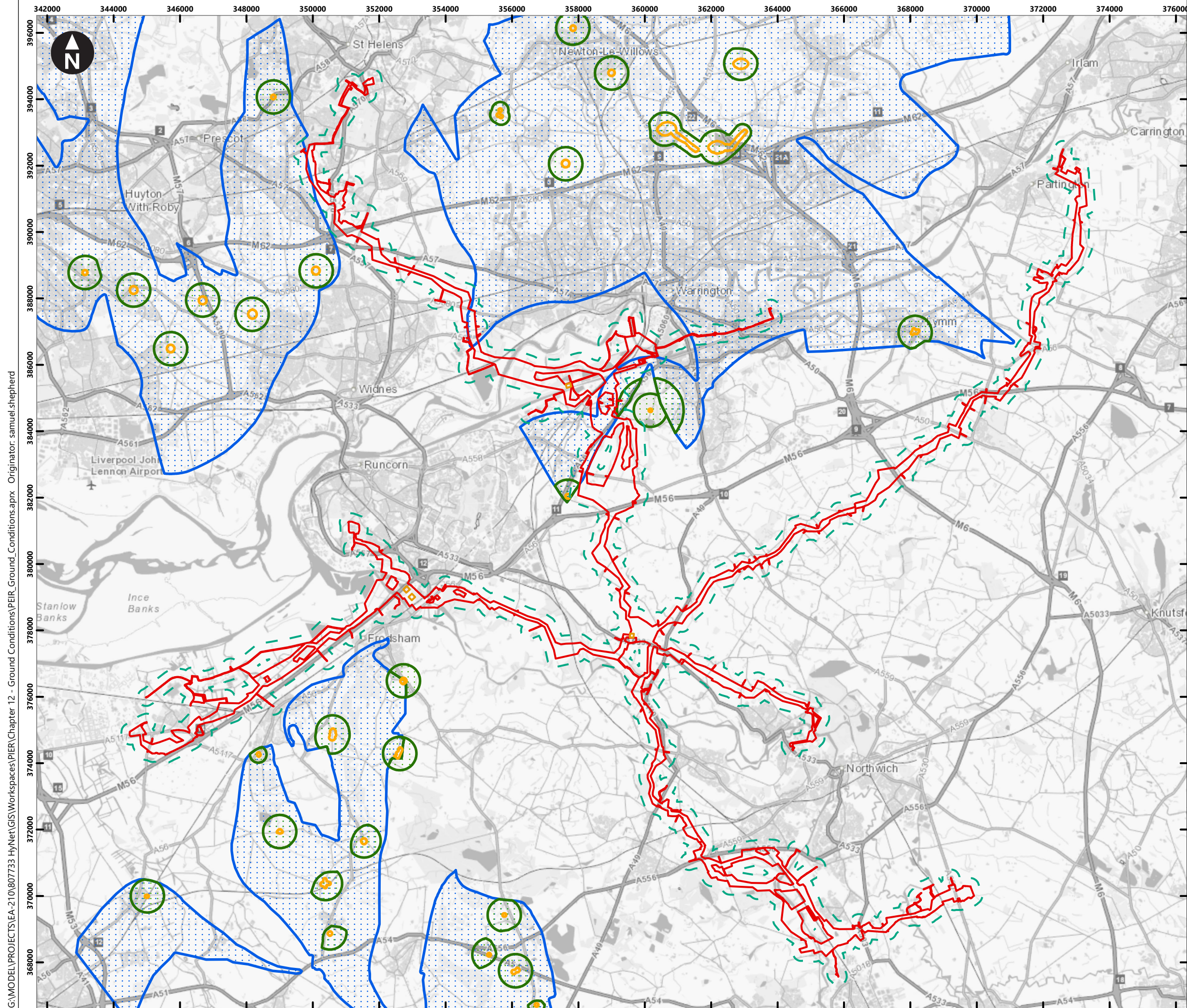
Figure 12.5 Groundwater Source Protection Zones
