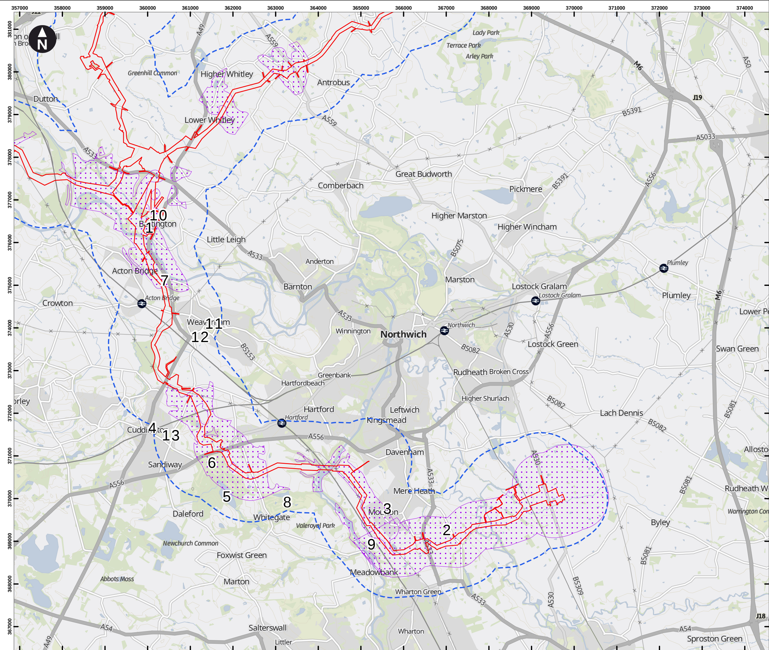
Figure 14.5 South Corridor Land Use Receptors
