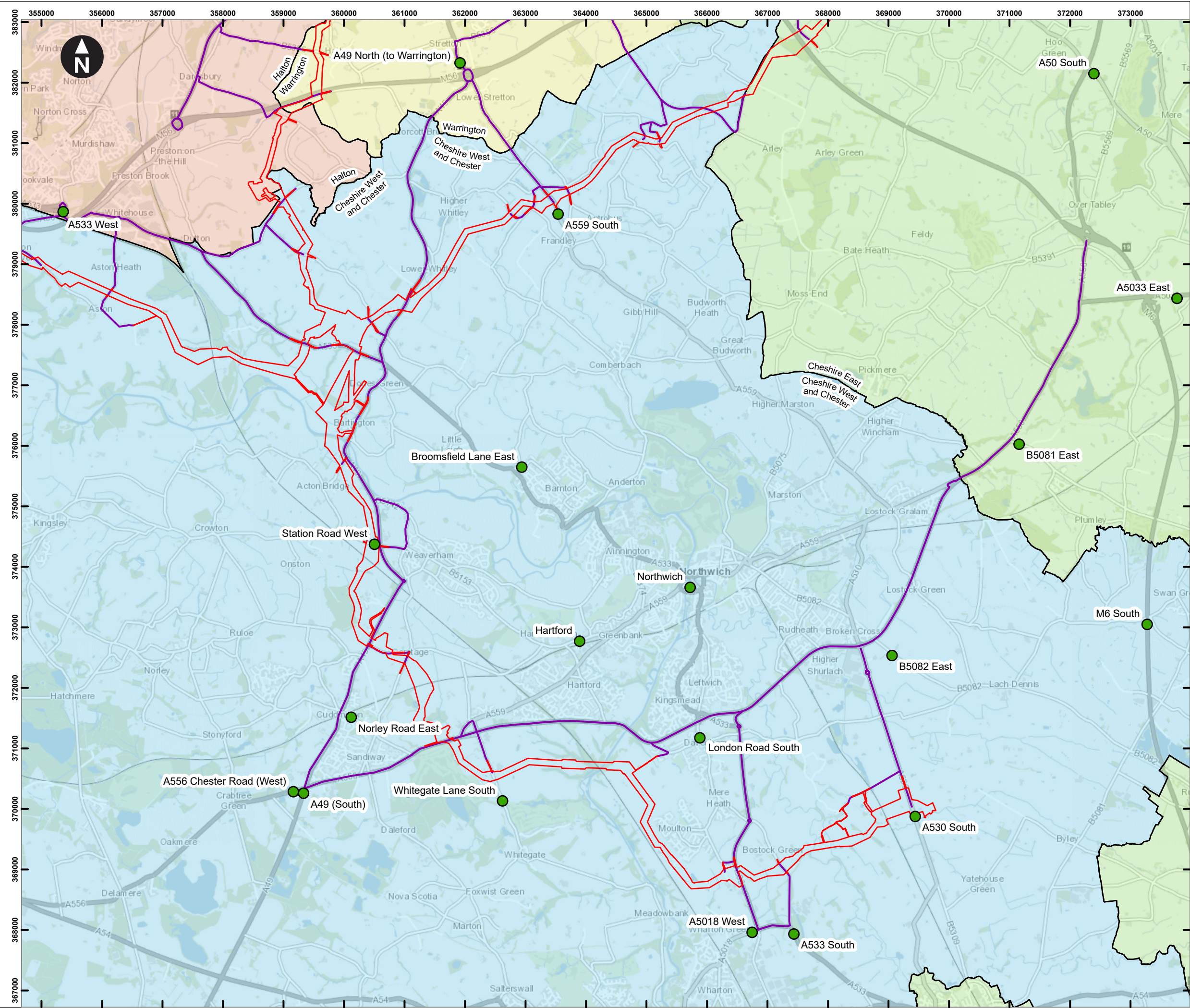
Figure 11.19 LV Distribution South
